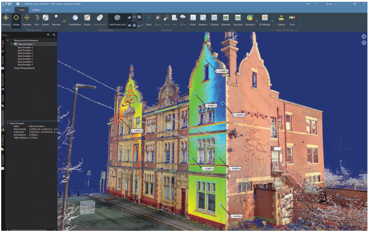
Point cloud rendering advancements have introduced new ways to work with the data. Evaluation of surface variance for condition monitoring and highlighting gradient is now possible.
