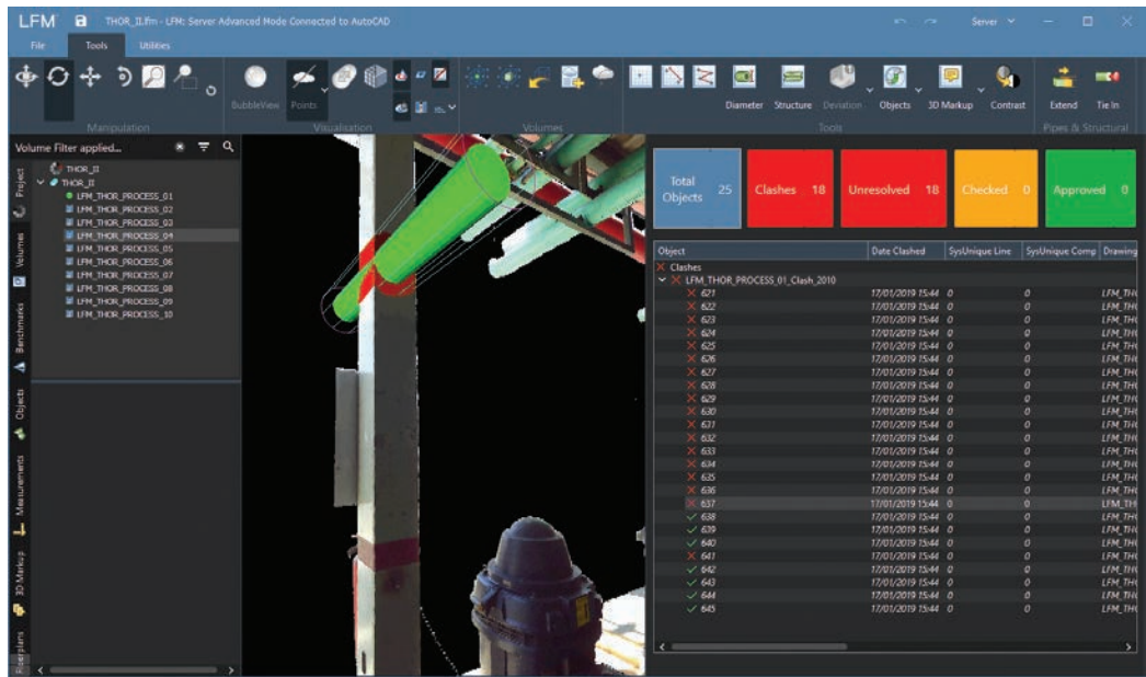
Design verification using the automated clash evaluation tools
