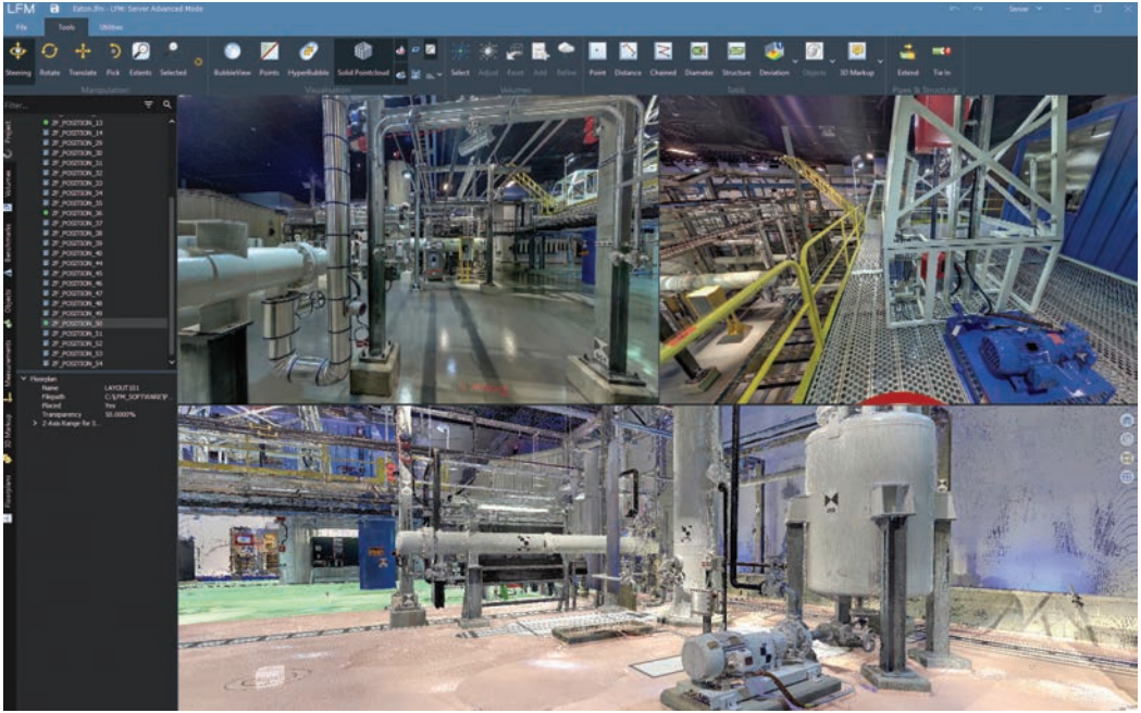
Integrated BubbleView and Solid Point Cloud
